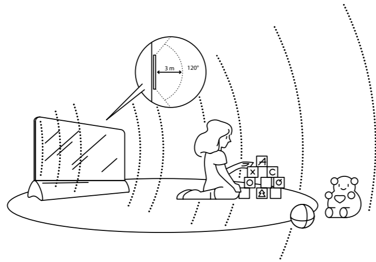
Figure 2. ThermoUp Floor/LED Plus heater radiation
